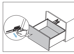
Press the locking device under drawer bottom and pull out the drawer
