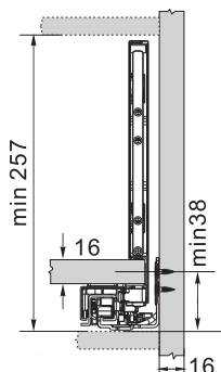
Space requirement in cabinet
