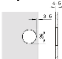
Drilling dimensions for cup fixing
