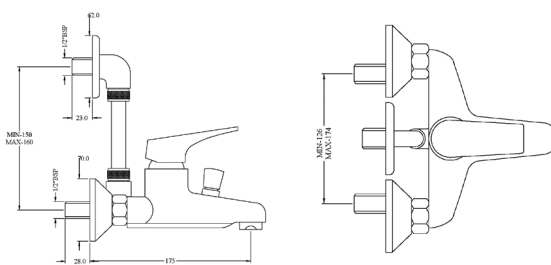
Single Lever Wall Mixer With L Bend 589.47.664 Chrome
