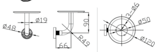
Soho Soap Dispenser
