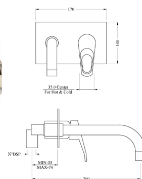
Single Lever Wall Mounted Basin Mixer - Concealed Part 589.47.816 Chrome
