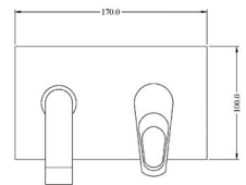
Single Lever Wall Mounted Tap - Concealed Part 589.47.817 Chrome
