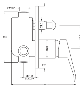
Single Lever Concealed Diverter (Bath And Shower) - Concealed Part 589.47.818 Chrome
