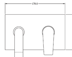
Single Lever Wall Mounted Tap - Concealed Part 589.47.817 Chrome
