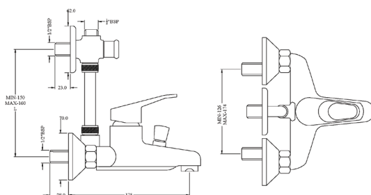
Single Lever 3-In-1 Wall Mixer With 'L' Bend 589.47.805 Chrome
