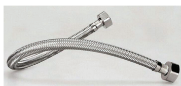
Connection Hose 450mm SS-304 braided with EPDM liner , 12 mm OD , SS nuts 1/2" 589.47.991
